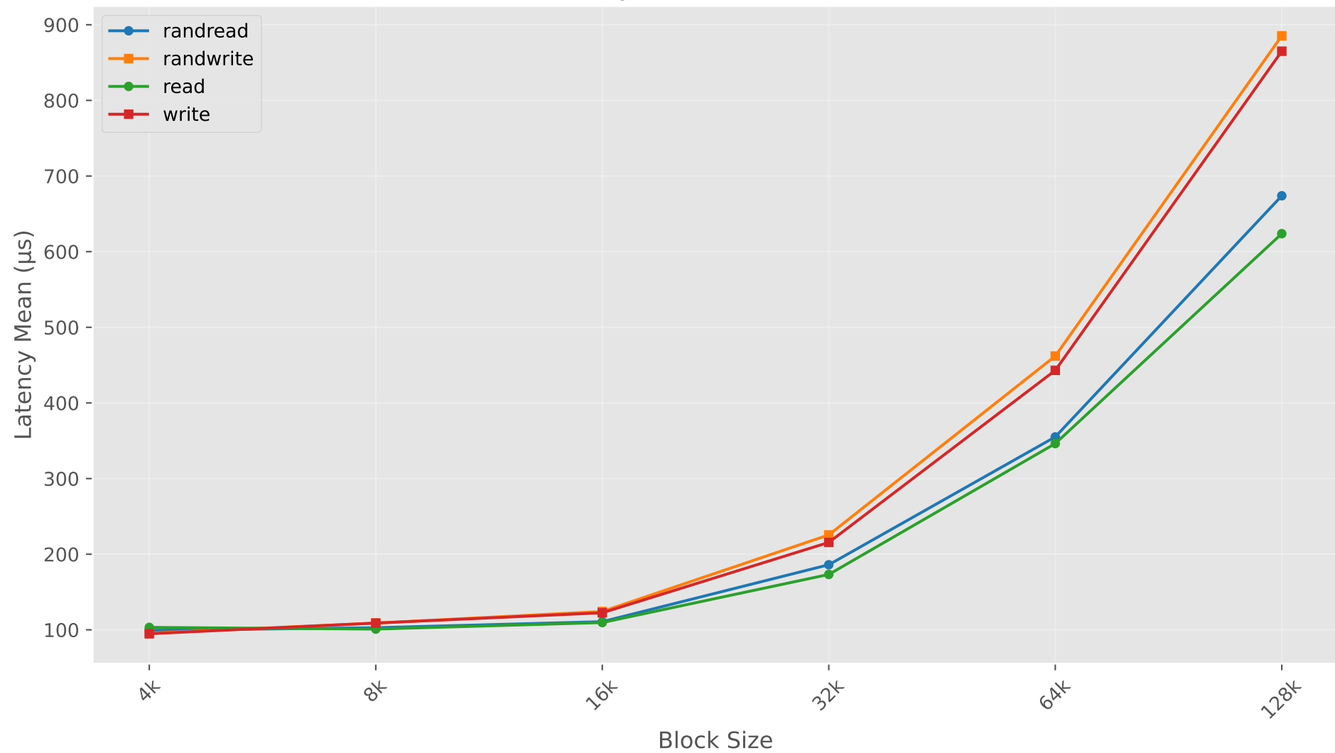
Latency Mean vs Block Size
